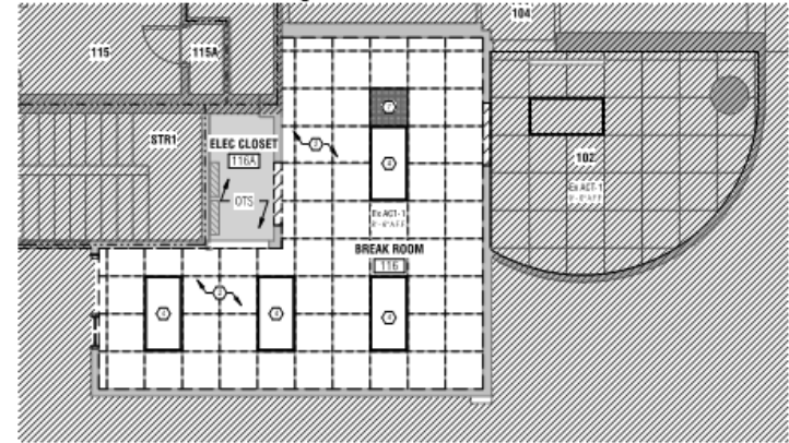
03 ENLARGED REFLECTED CEILING PLAN 1/8" = 1'-0"
