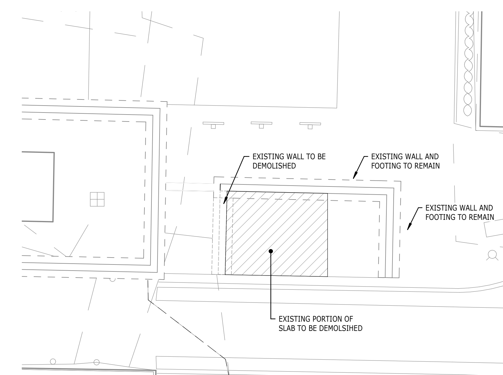
2 DEMO PLAN S100 1/8" = 1'-0"
