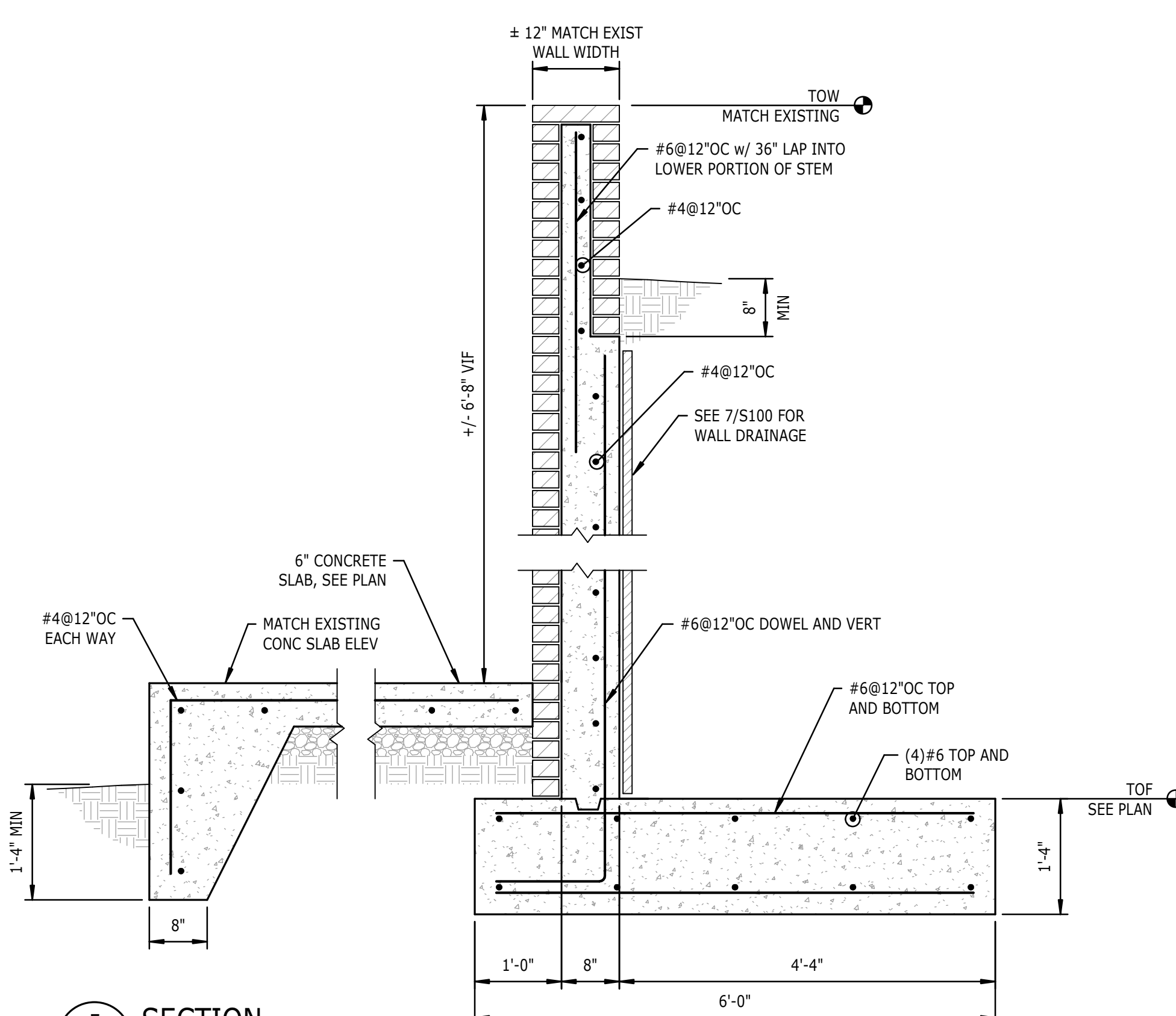
5 SECTION S100 3/4" = 1'-0"
