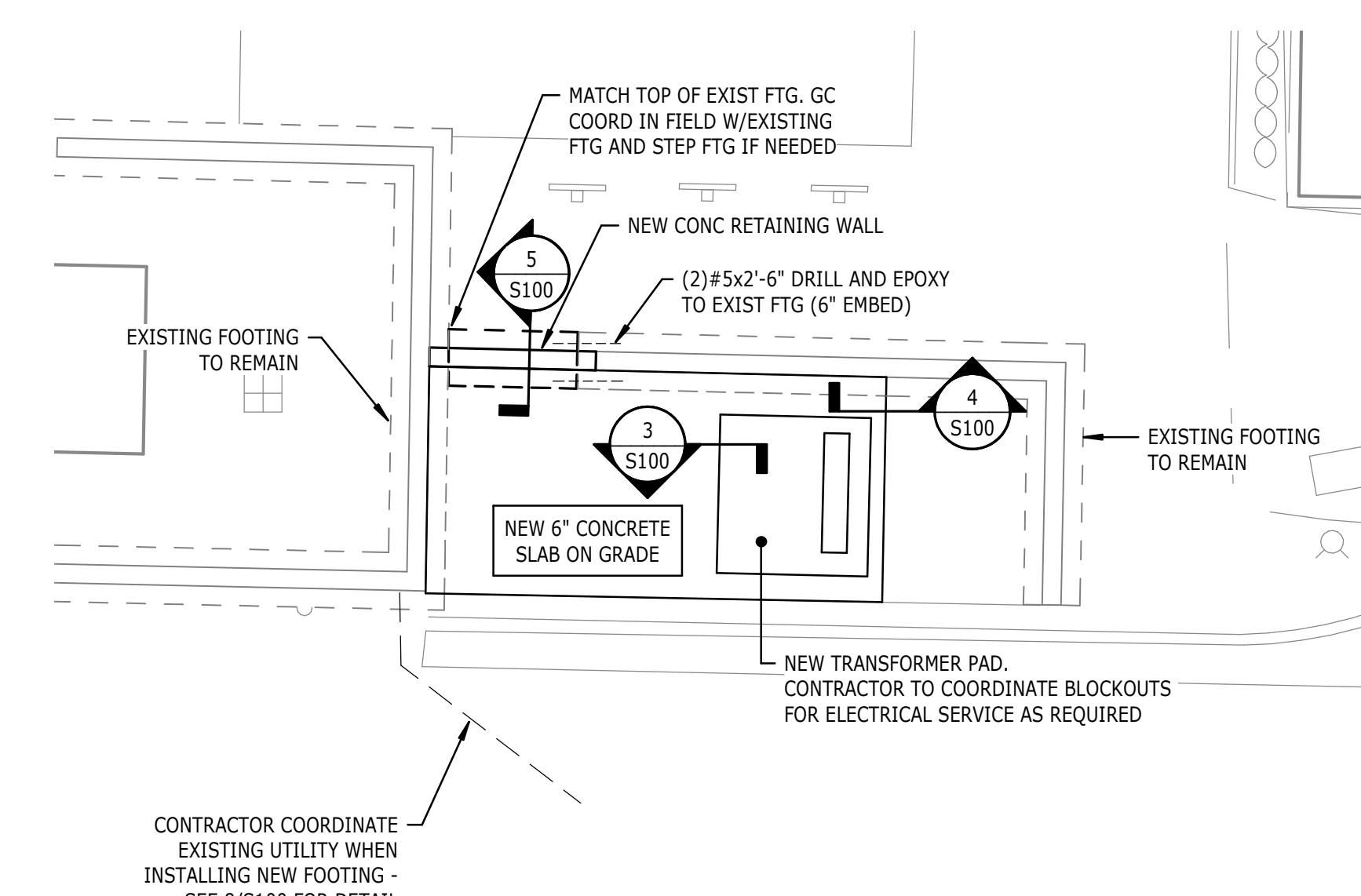
1 FOUNDATION PLAN S100 1/8" = 1'-0"
