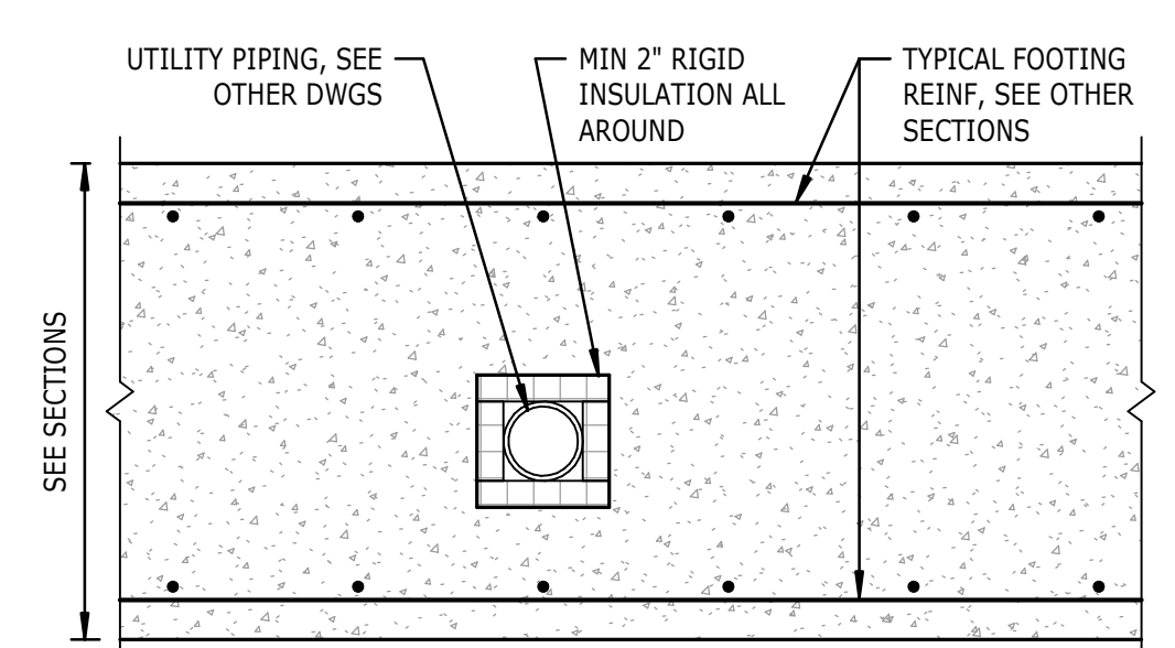
PIPE IN FOOTING
