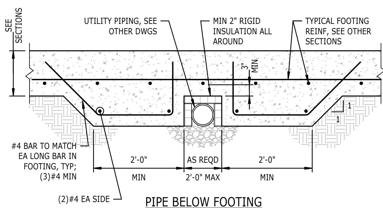
PIPE BELOW FOOTING
